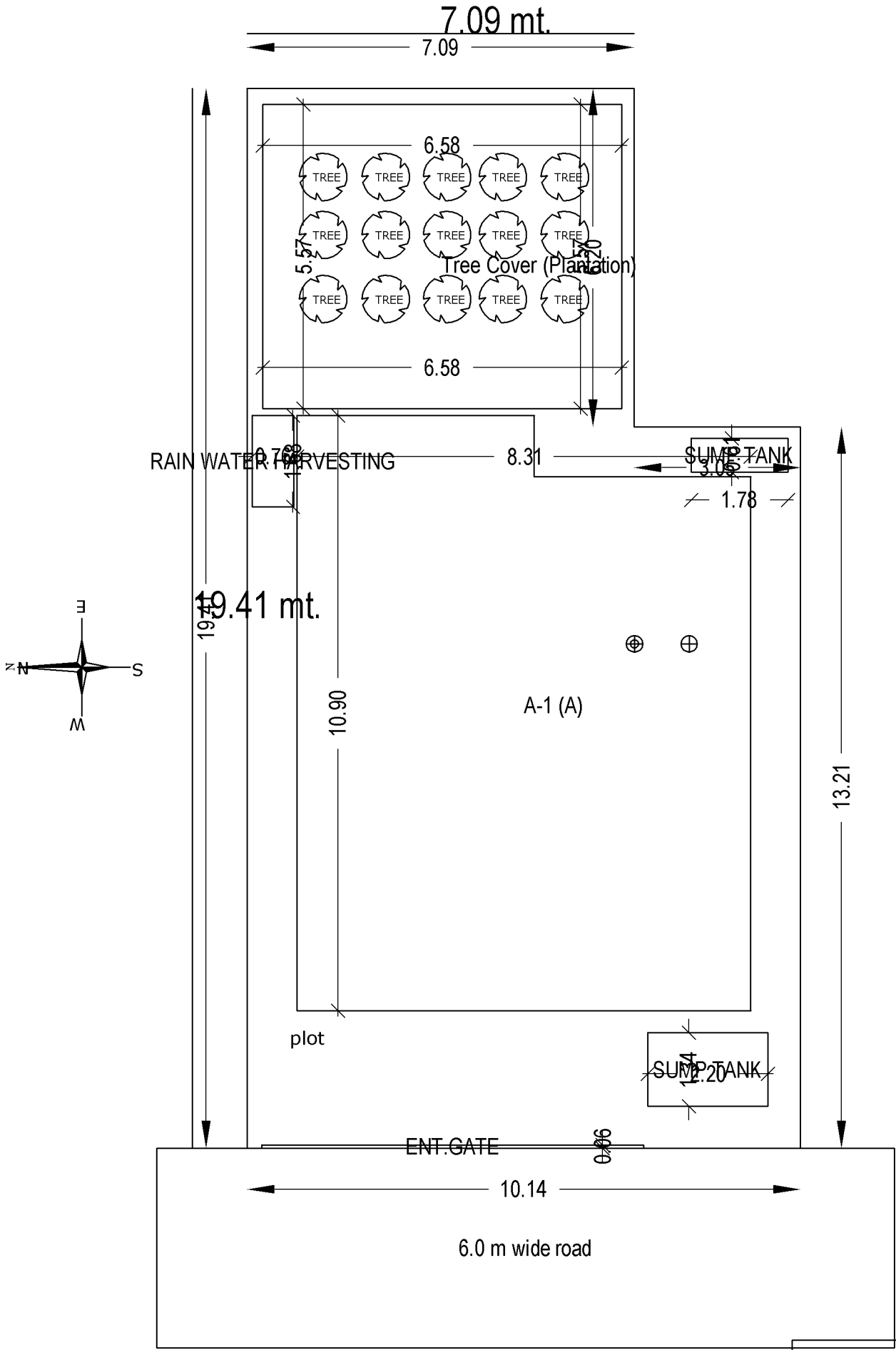
site plan
