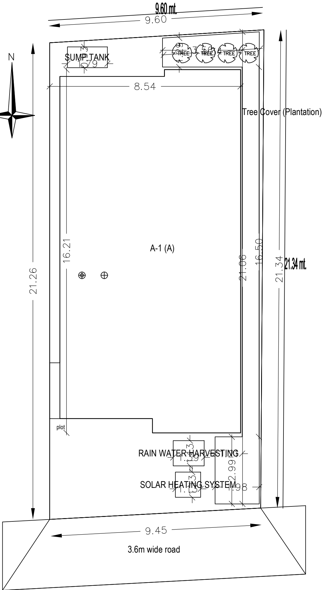
site plan
