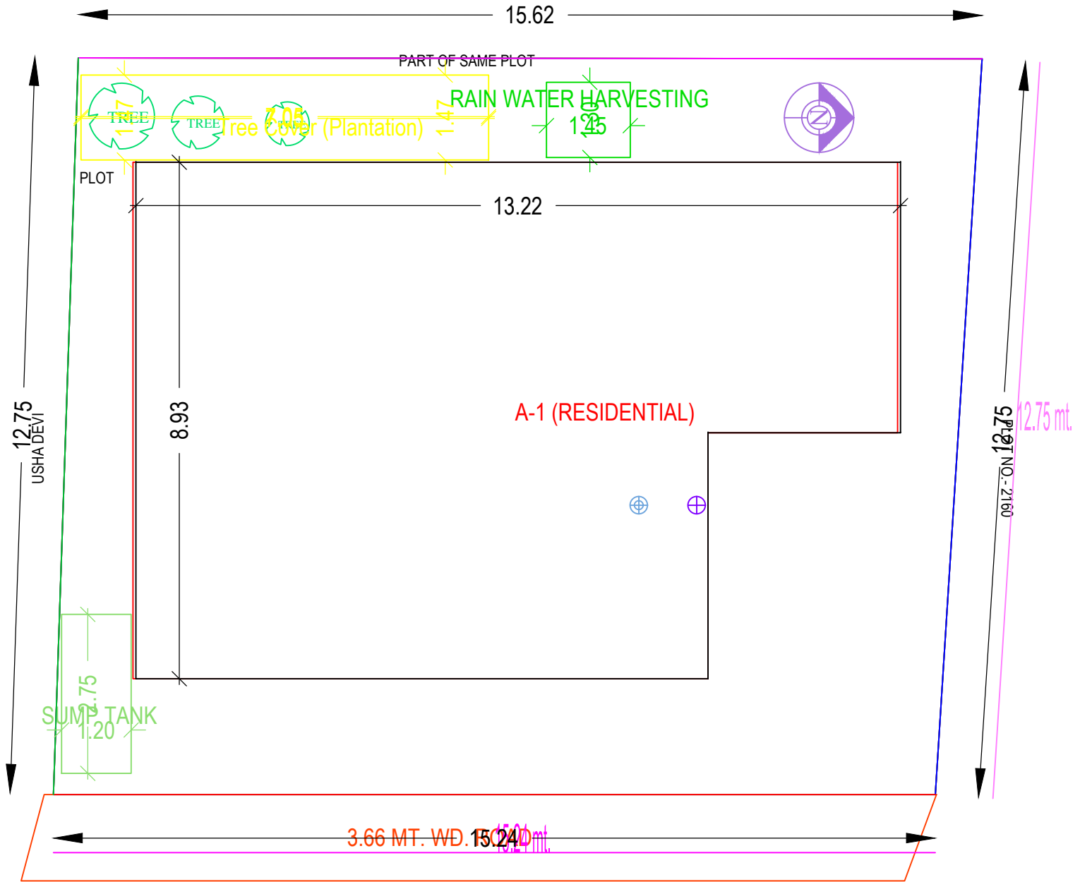
SITE PLAN
