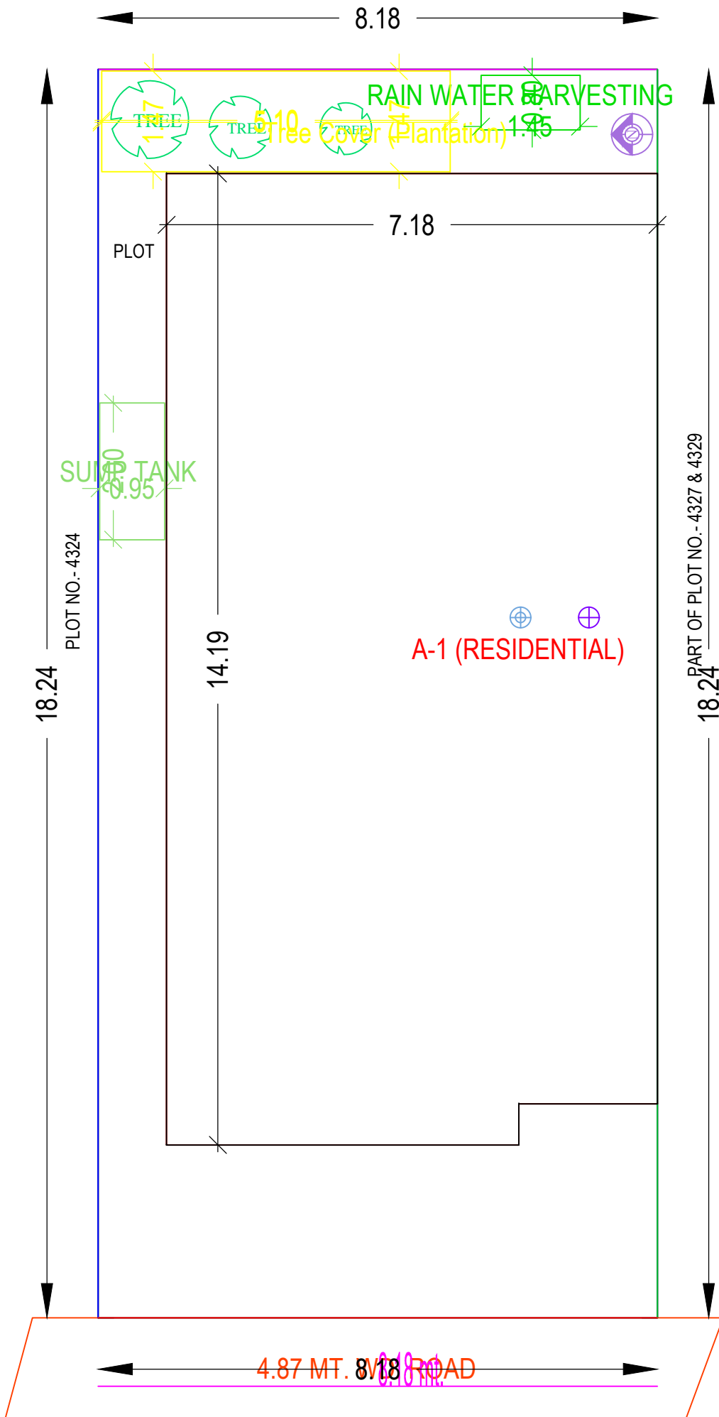
SITE PLAN
