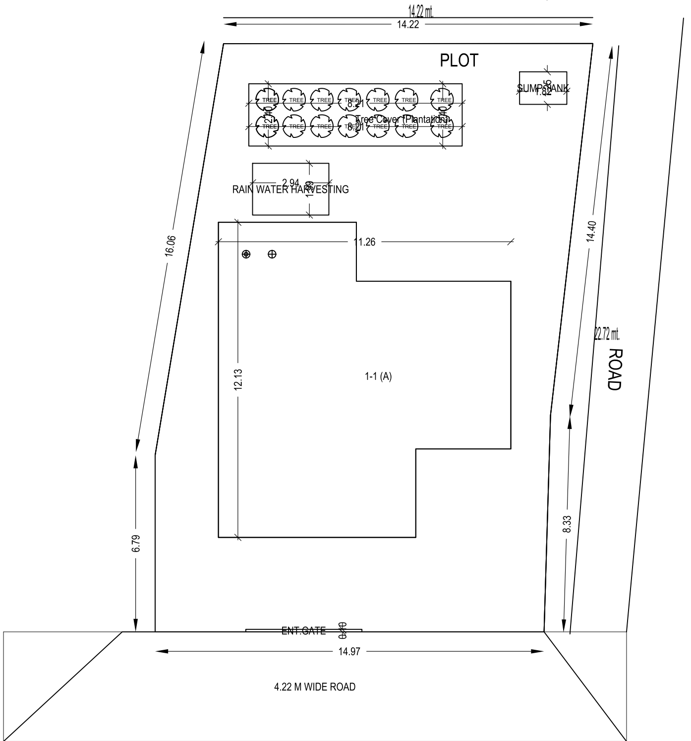
SITE PLAN
