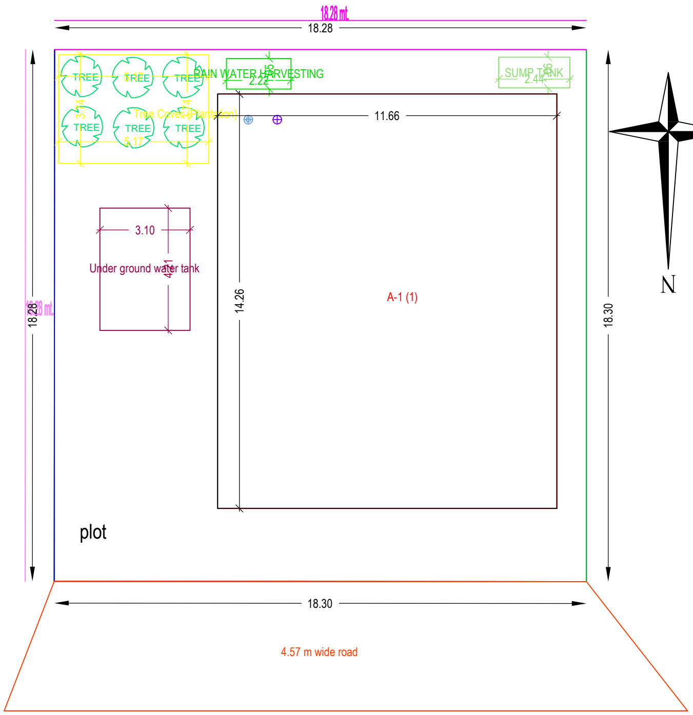
site plan
