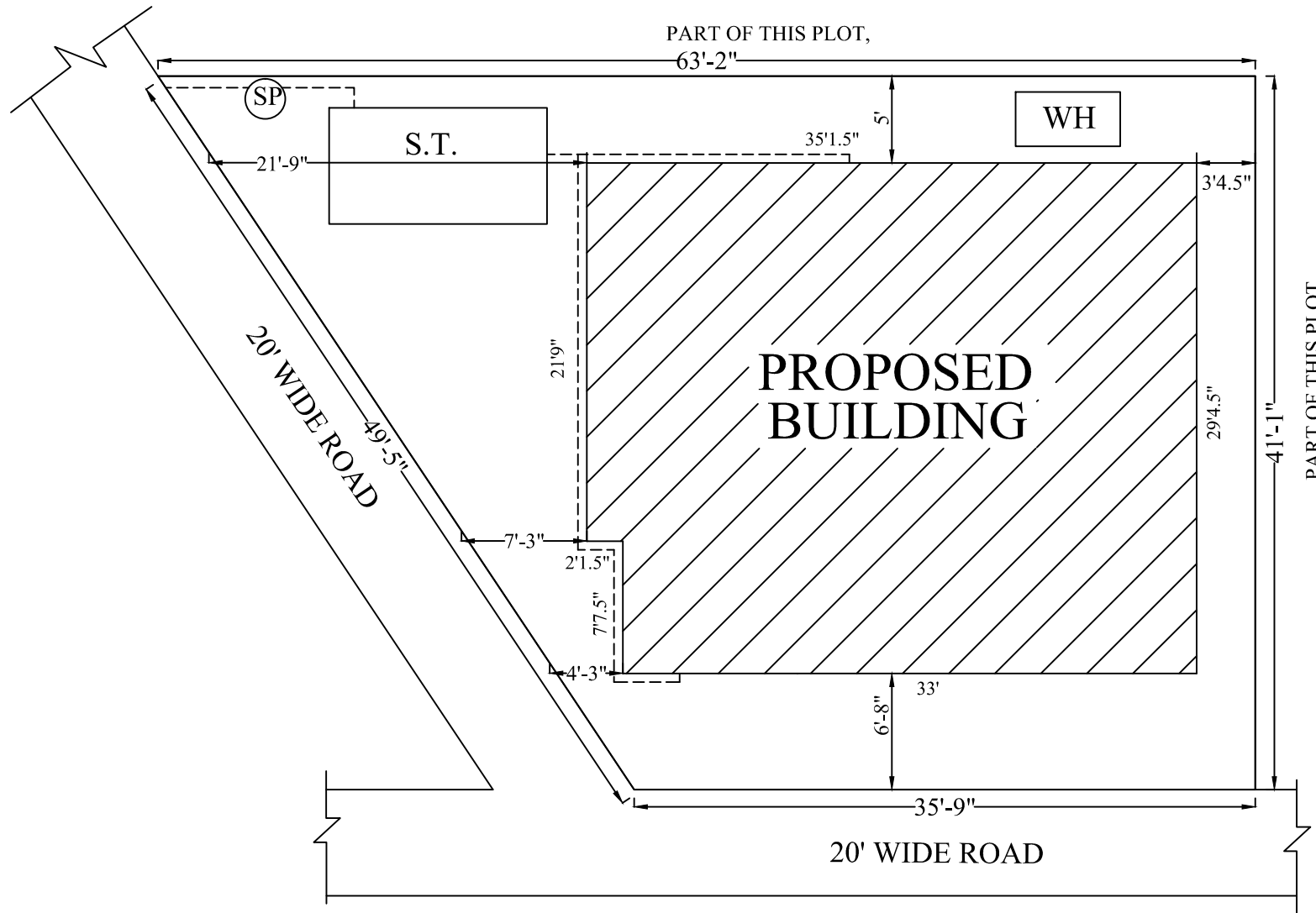
SITE PLAN
