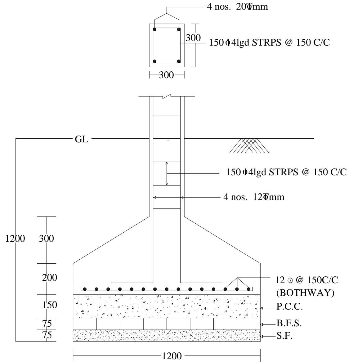
SECTION
