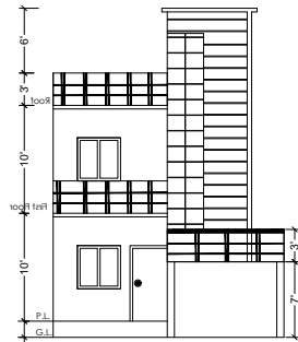
Front Elevation SCALE 1:100
