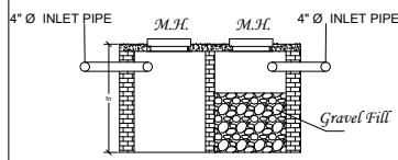
SECTION OF X-X SCALE 1:50
