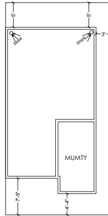
TERRACE FLOOR PLAN SCALE 1:100
