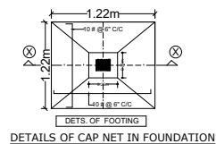
DETAILS OF CAP NET IN FOUNDATION
