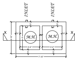
SOAK PIT PLAN SCALE 1:50
