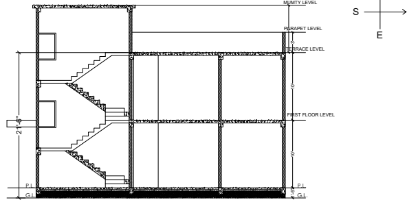
SECTION: X-X SCALE 1:100
