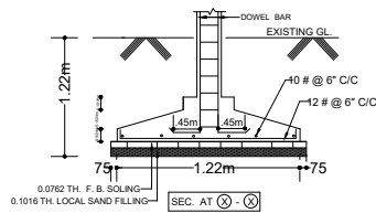
DETAILS OF CAP NET IN FOUNDATION
