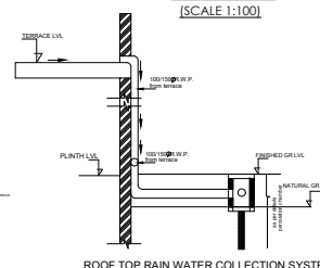
ROOF TOP RAIN WATER COLLECTION SYSTEM
