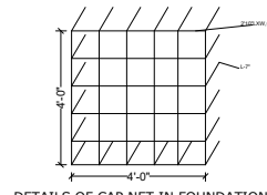
DETAILS OF CAP NET IN FOUNDATION
