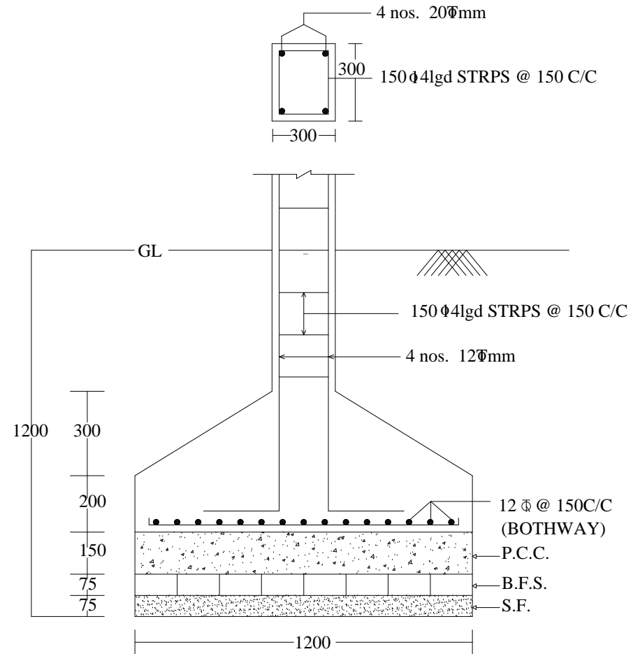
SECTION
