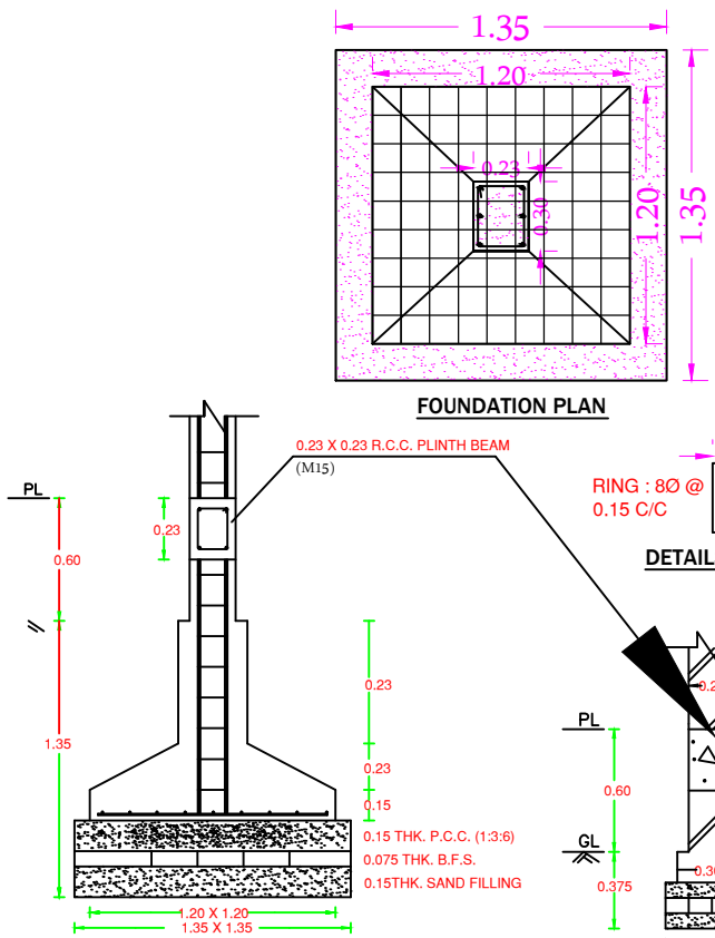
FOUNDATION DETAILS OF COLUMN
