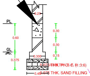
FOUNDATION DETAILS OF WALL
