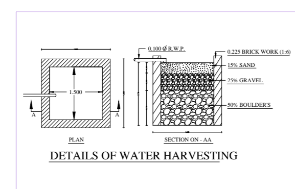
DETAILS OF WATER HARVESTING
