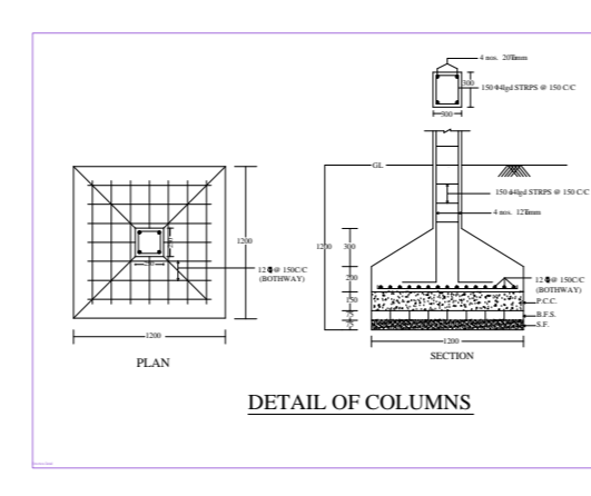
DETAIL OF COLUMN
