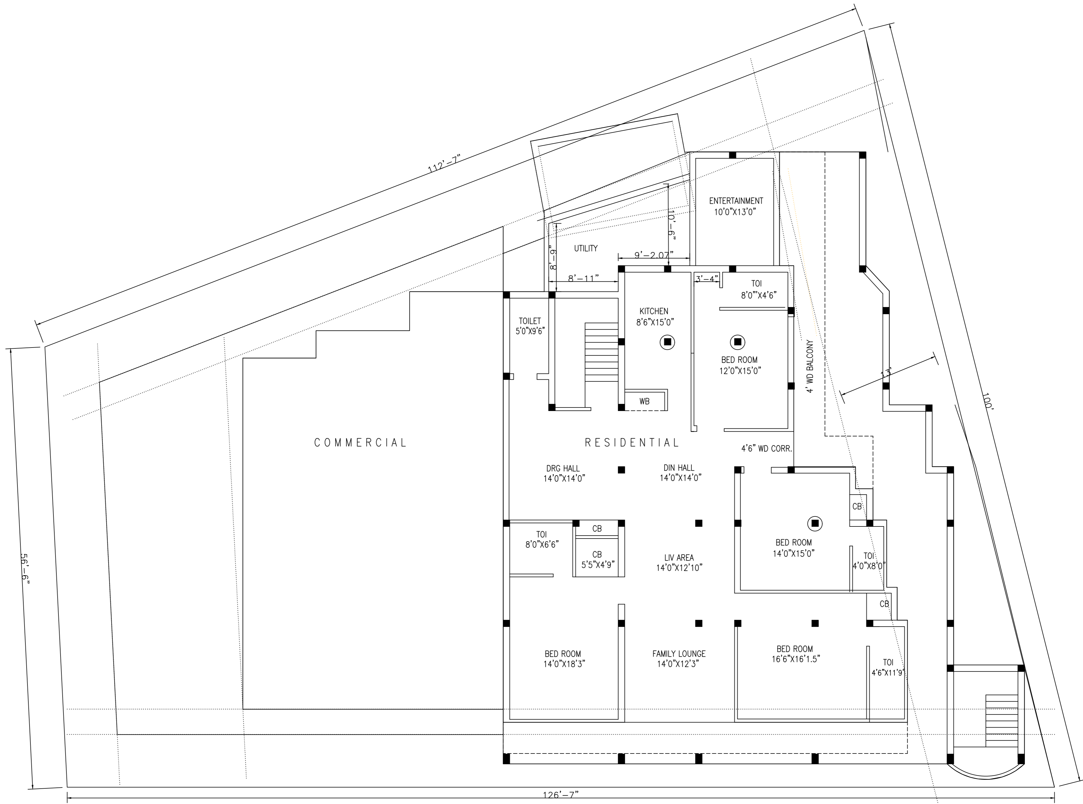
SECOND FLOOR PLAN (RES)
