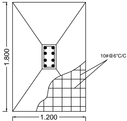
COLUMN DETAILS SCALE:- 1:50
