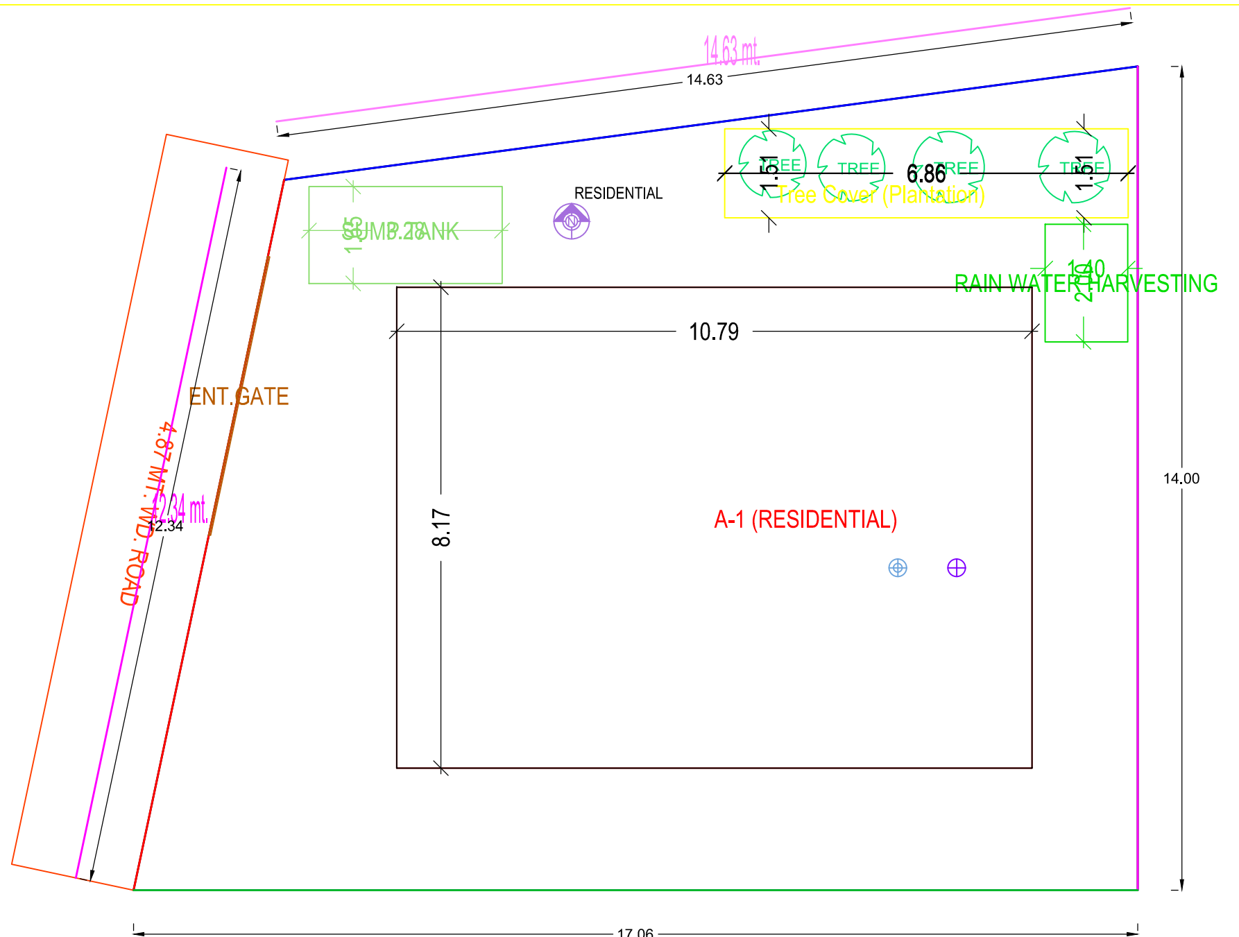
SITE PLAN
