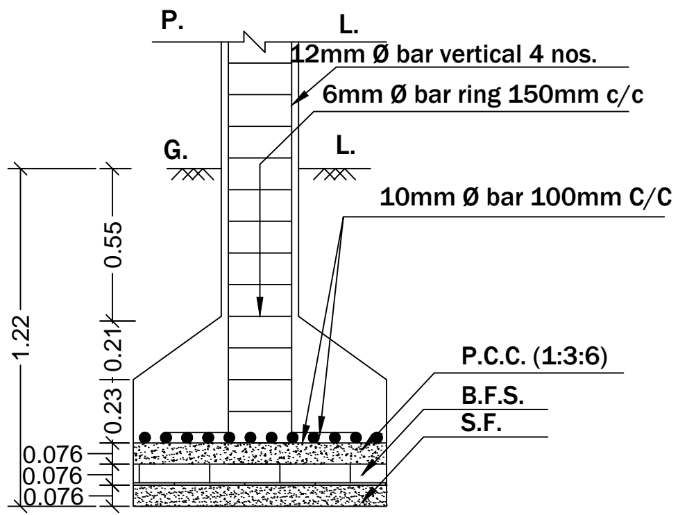
SECTION ON- ZZ SCALE - 1:25
