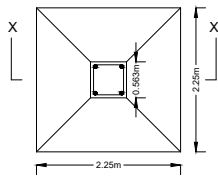
DETAILS OF COLUMN FOUNDATION SCALE - 1:100
