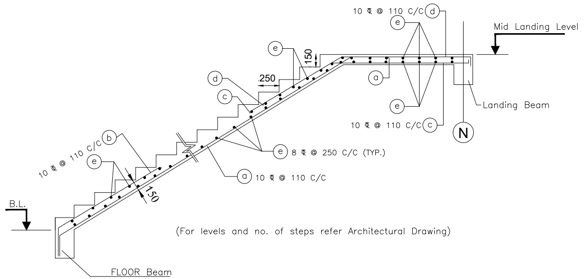
TYP. DETAIL OF STAIR
