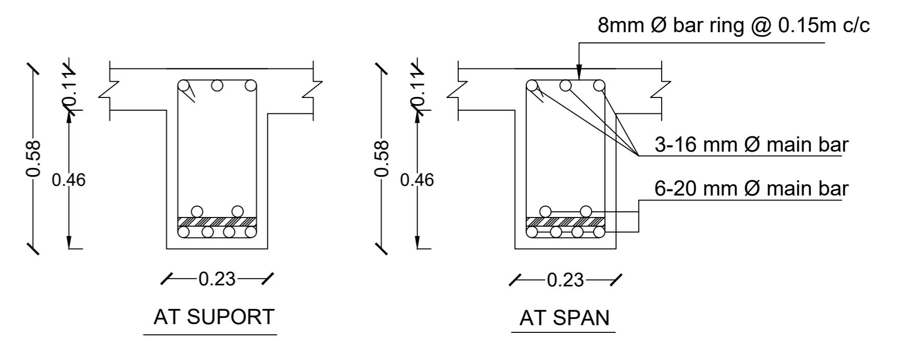
DETAILS OF TYPICAL ROOF BEAM
