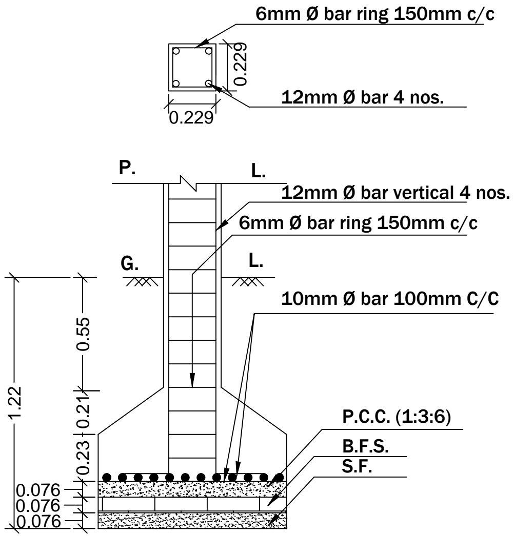
SECTION ON- ZZ SCALE - 1:25
