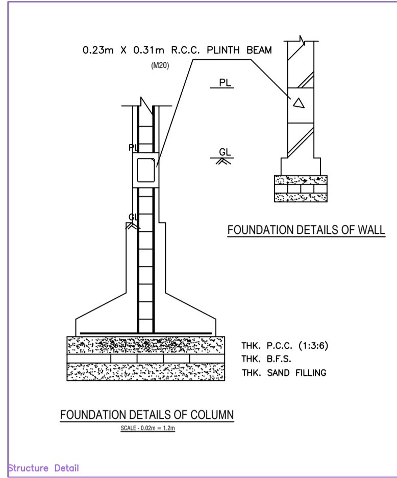
Structure Detail
