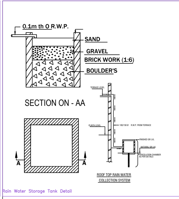
Rain Water Storage Tank Detail
