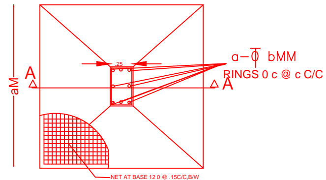
PLAN OF COLUMN FOUNDATION
