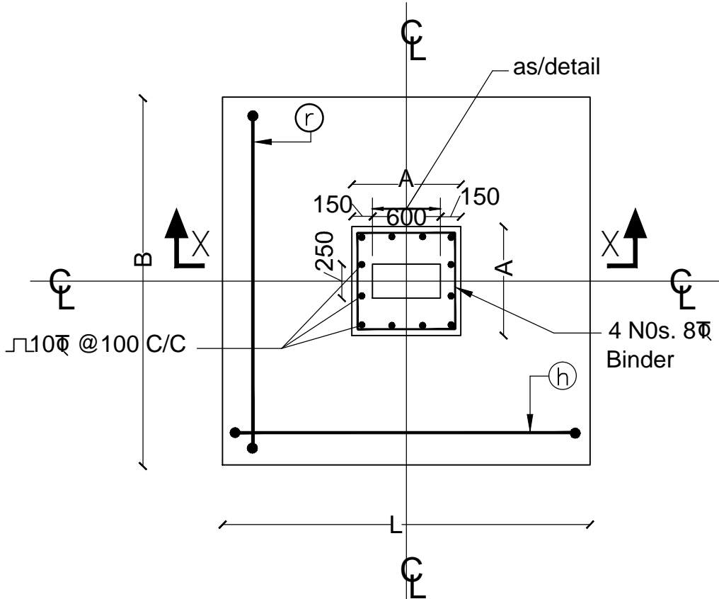
TYP DETAIL OF FOOTING
