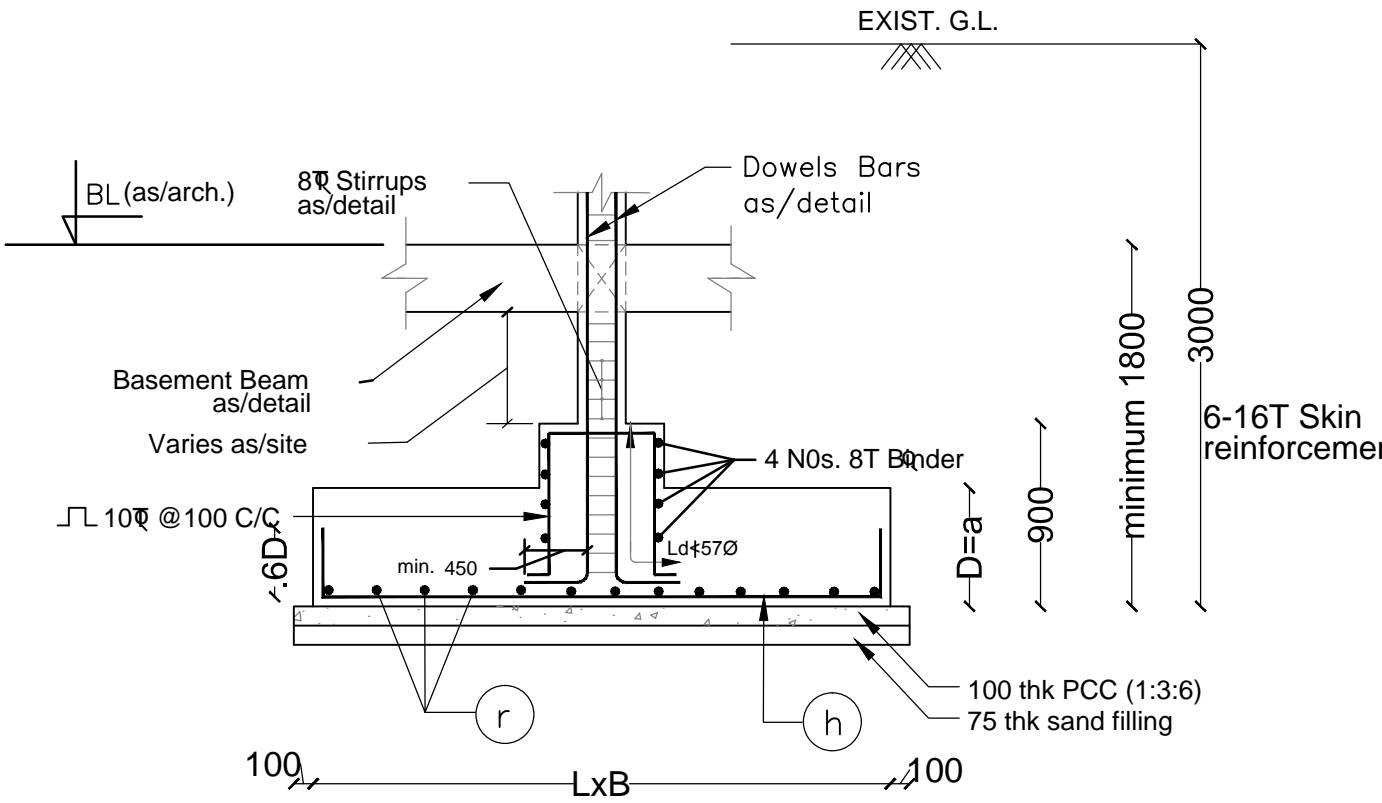
SECTION X-X
