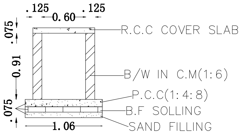
SECTION OF DRAIN
