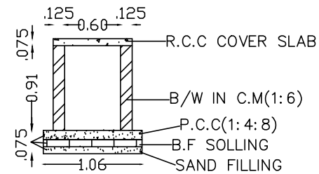
SECTION OF DRAIN
