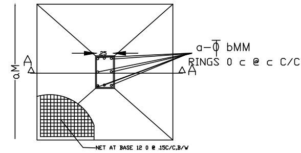
PLAN OF COLUMN FOUNDATION
