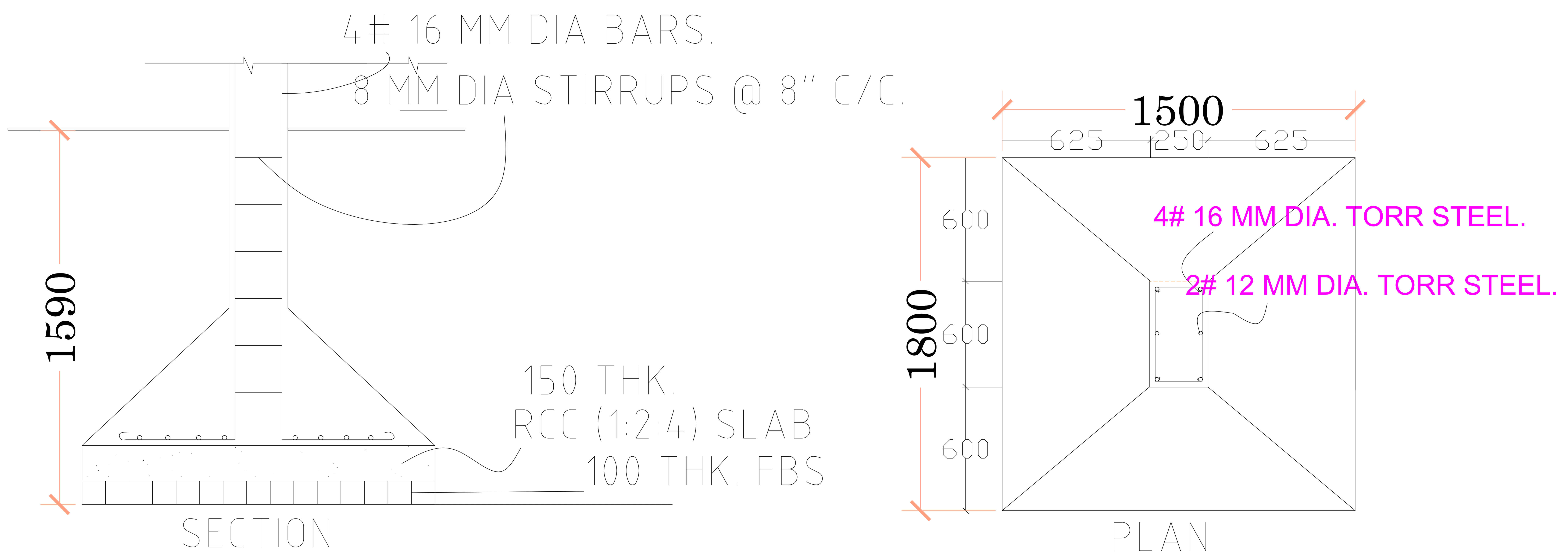
FOUNDATION DETAILS (ISOLATED R.C.C FOOTING)
