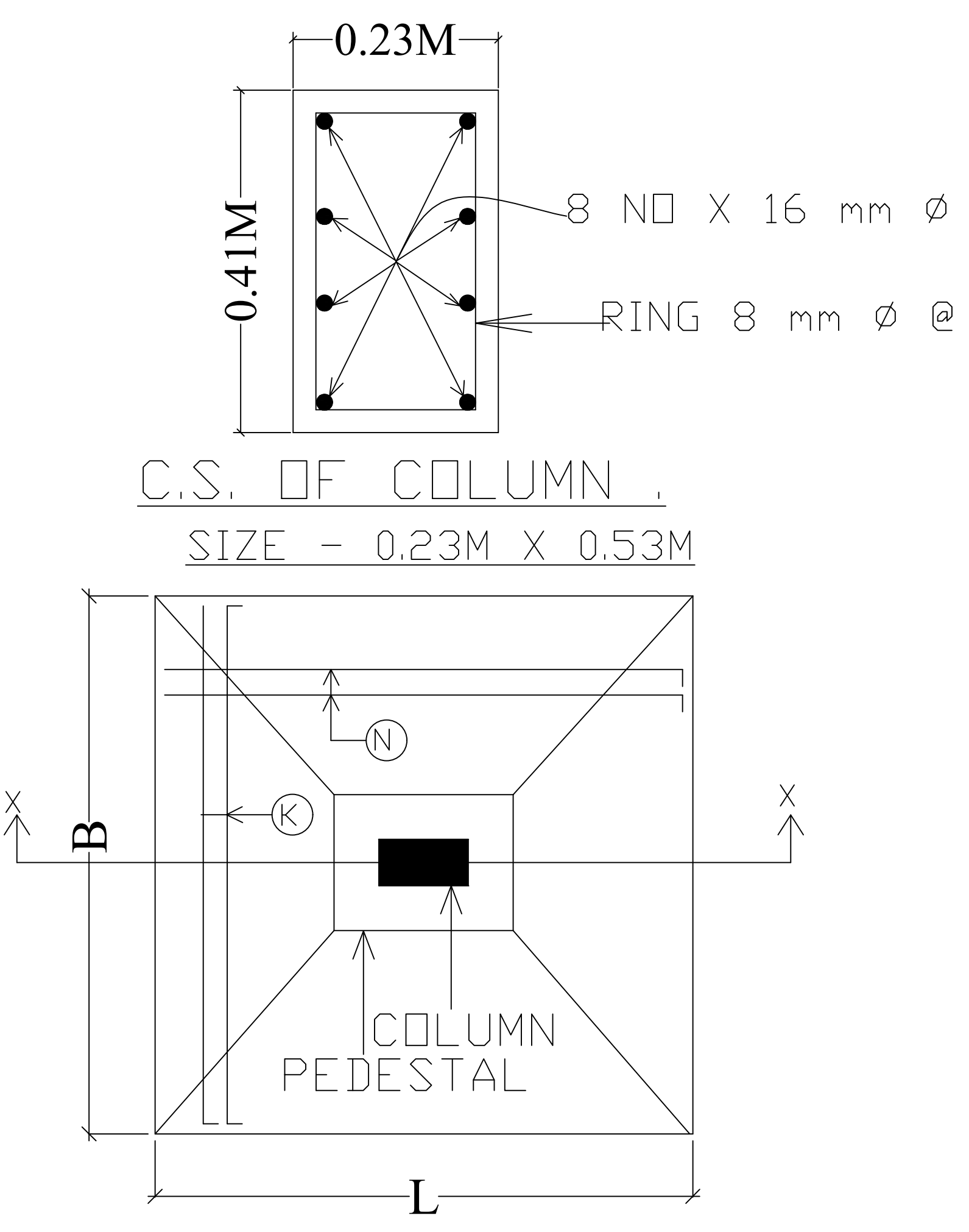
PLAN OF ISOLATED FOOTING
