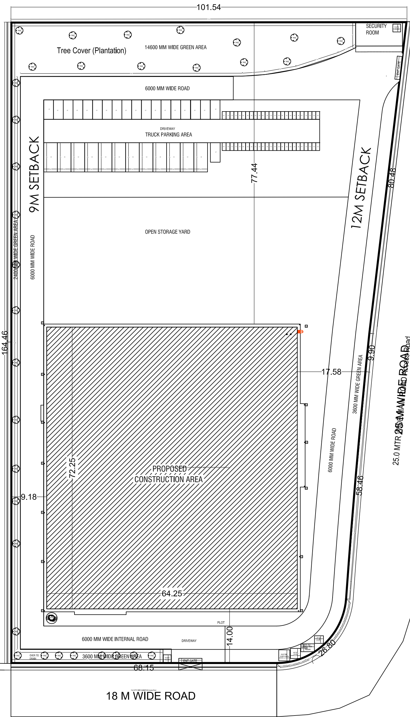
SITE CUM DRAINAGE PLAN (SCALE 1:500)
