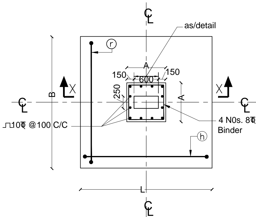
TYP DETAIL OF FOOTING
