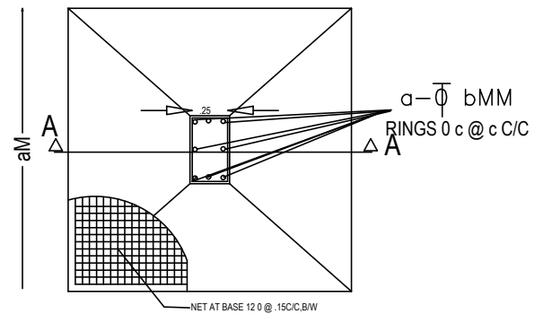
PLAN OF COLUMN FOUNDATION
