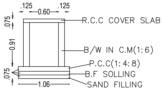
SECTION OF DRAIN
