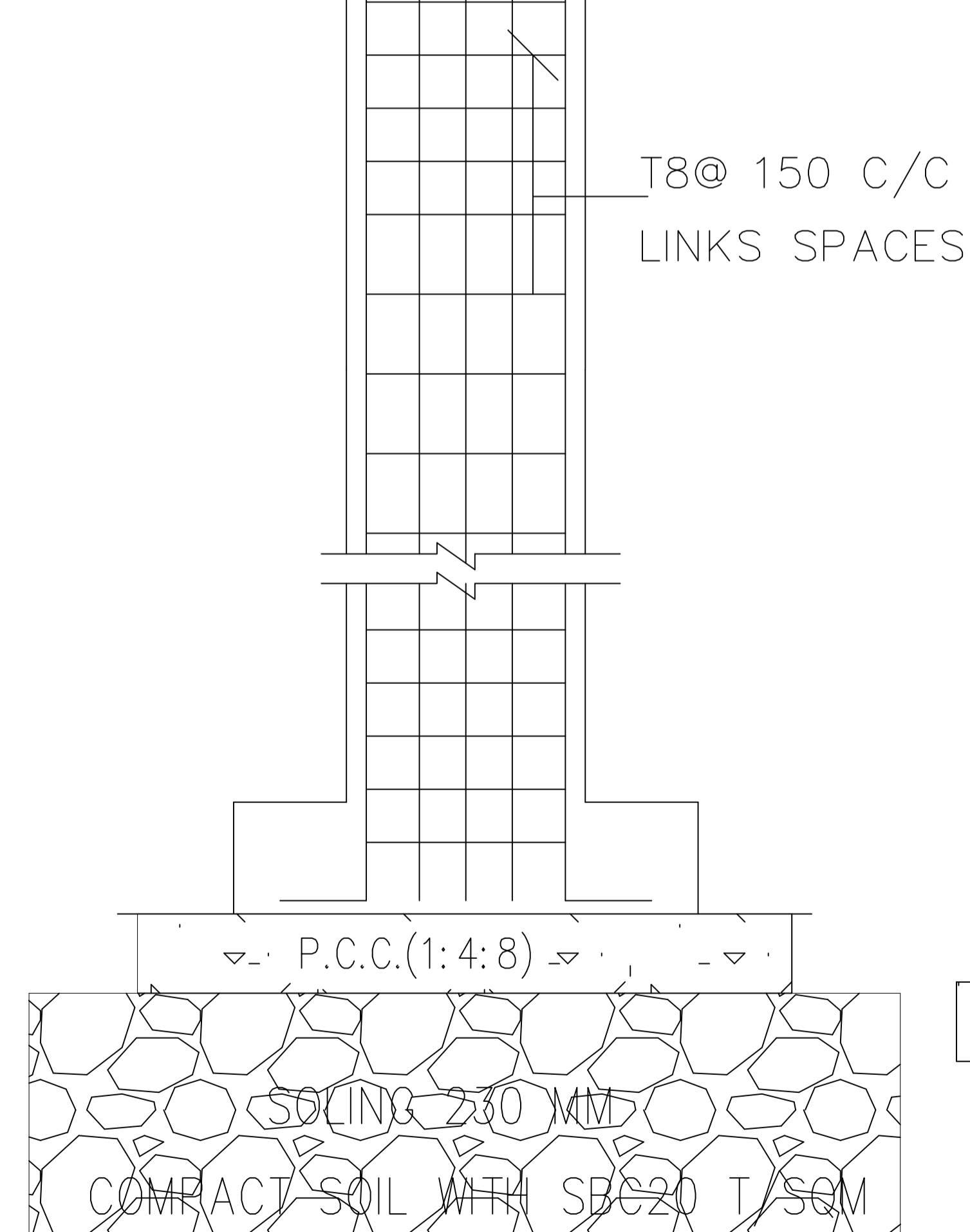
TYP. COLUMN LINKS DETAILS
