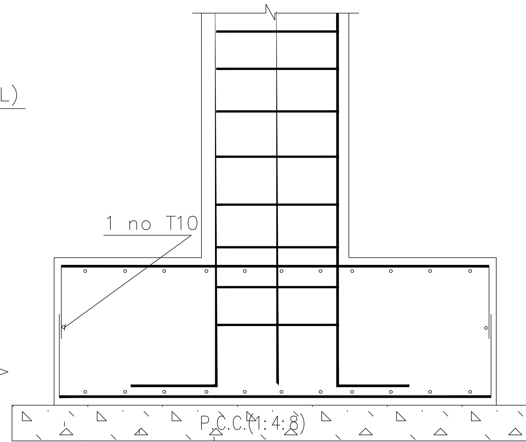
TYP. COL. FOOTING DETAIL. WITH TOP JALI
