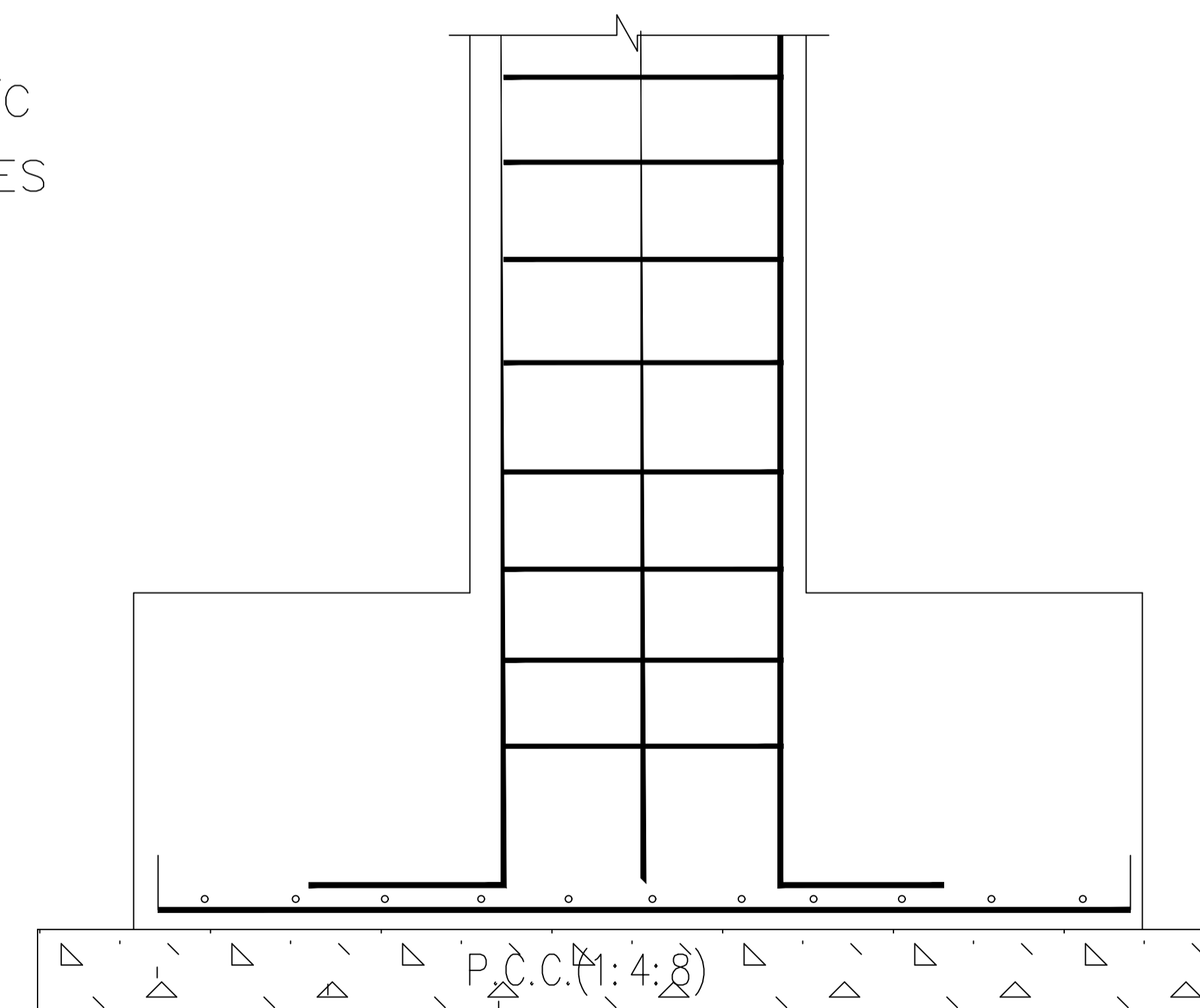
TYP. COL. FOOTING DETAIL. WITHOUT TOP JALI
