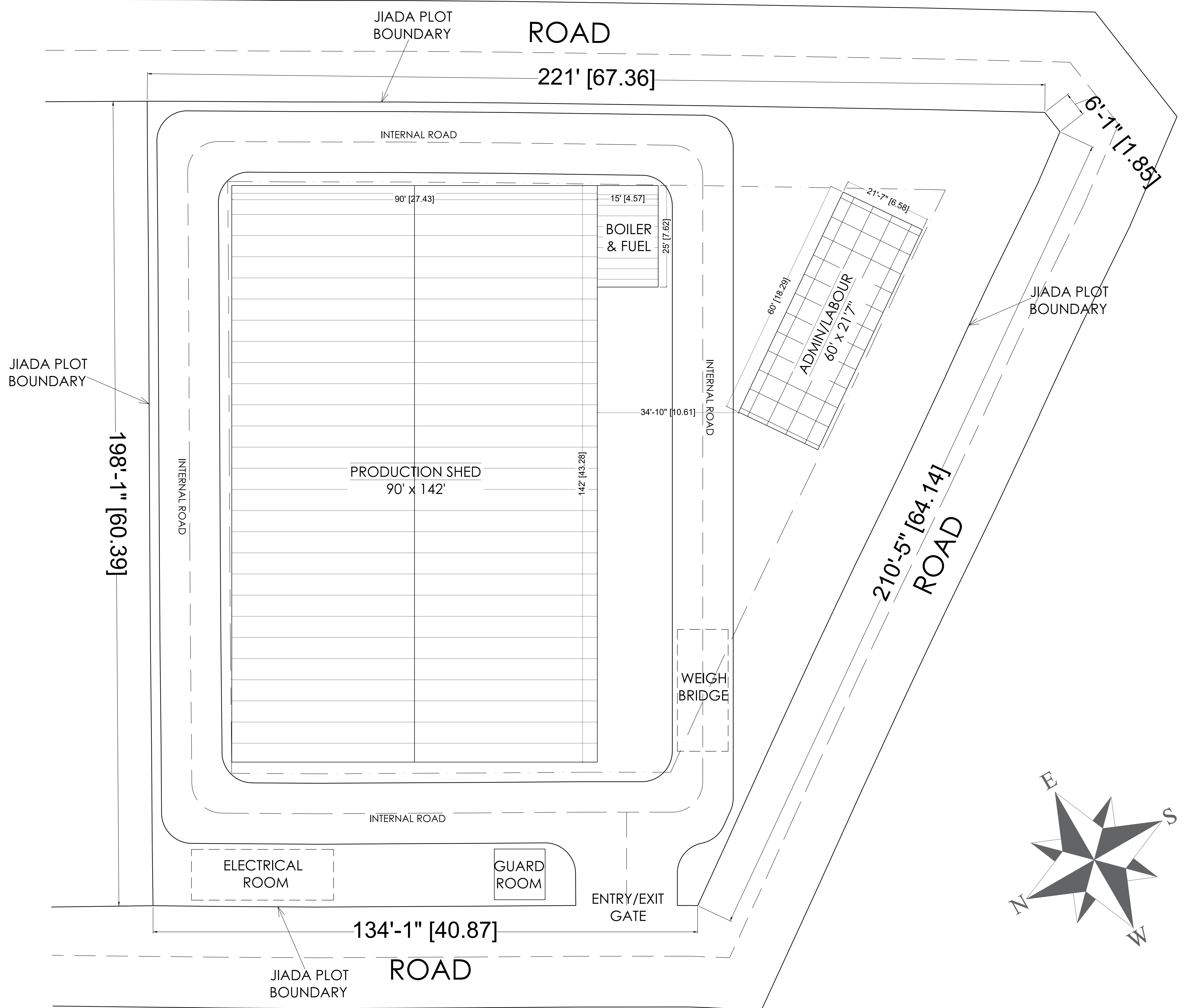
SITE LAYOUT PLAN
