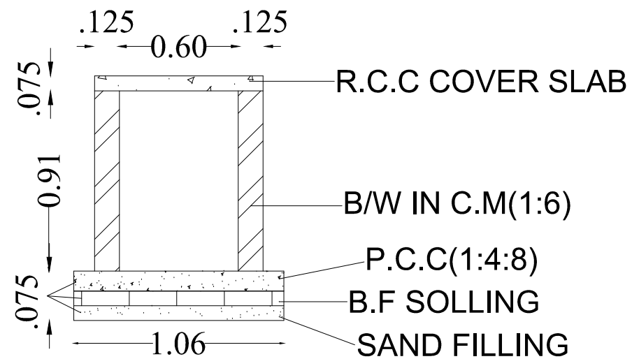
SECTION OF DRAIN
