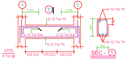
DET. OF SB1/PB1 (250X300)
