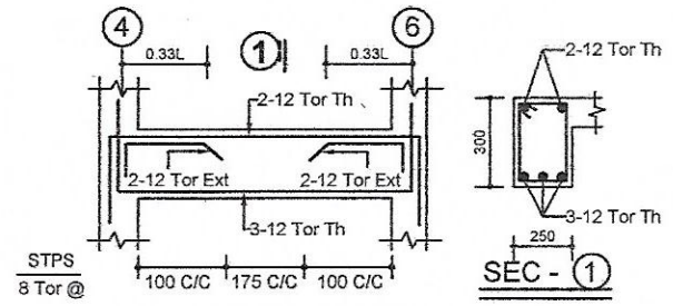
DET. OF SB1/PB1 (250X300)
