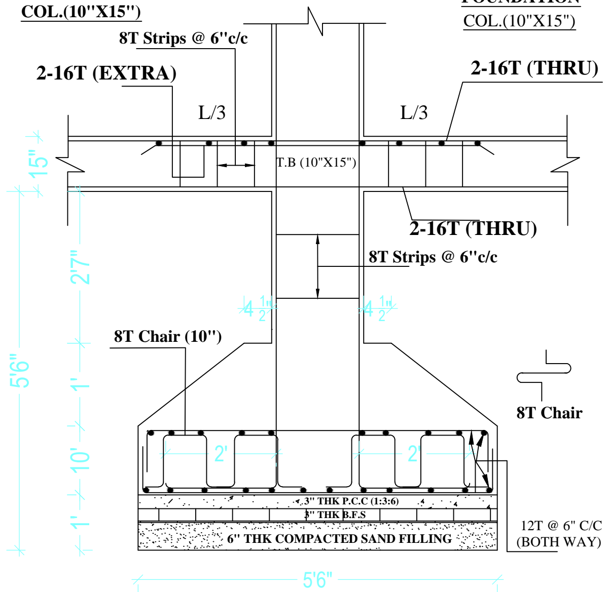
SECTION - B-B
