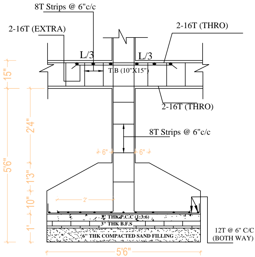
SECTION - B-B
