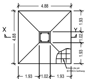
DETAILS OF 250 x 250 R.C.C. COLUMN FOUNDATION 1:50
