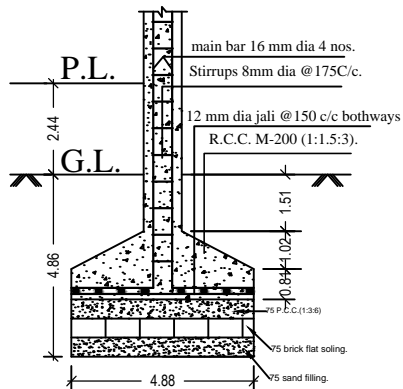
SECTIONAL ELEVATION
