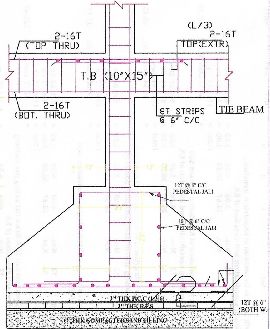
FOUNDATION COL. (10'X20')
