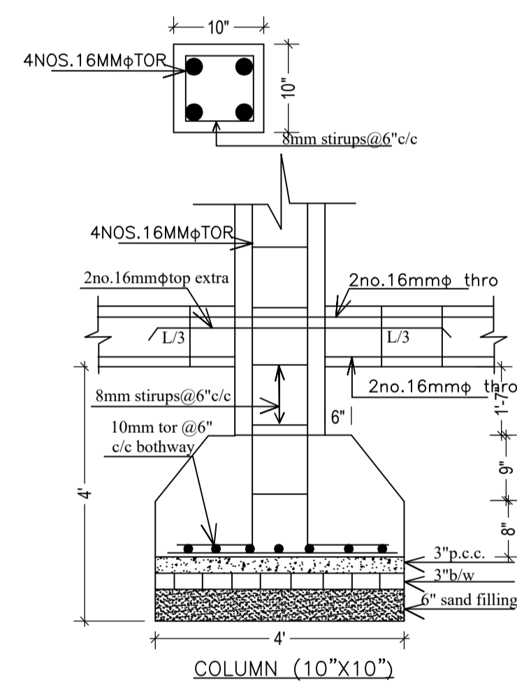
COLUMN (10"X10")
