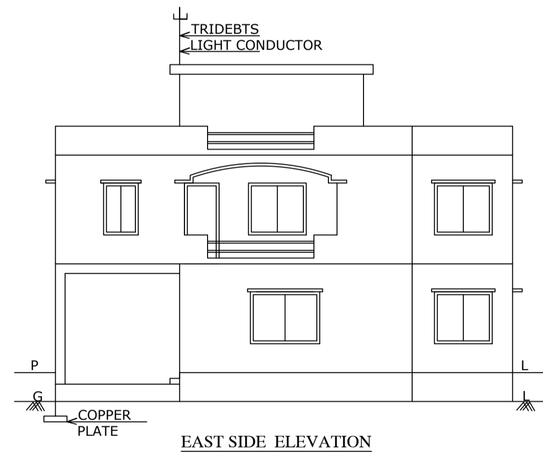
EAST SIDE ELEVATION
