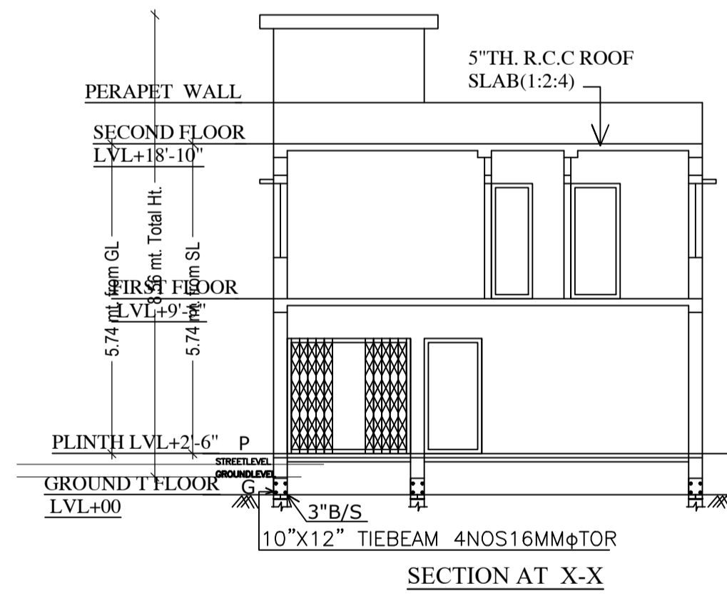
SECTION AT X-X
