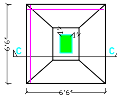
FOUNDATION COL. (10" x 20")
