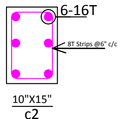
SECTION - B-B C2
