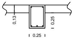
CROSS SECTION OF BEAM AT MIDDLE SPAN
