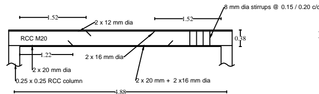
LONGITUDINAL SECTION OF ROOF BEAM
