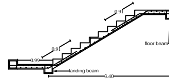
LONGITUDINAL SECTION 2ND FLIGHT
