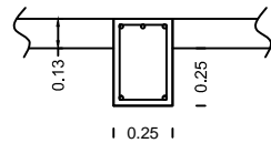
CROSS SECTION OF BEAM AT END SUPPORT
