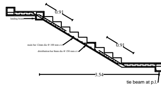
LONGITUDINAL SECTION 1ST FLIGHT
