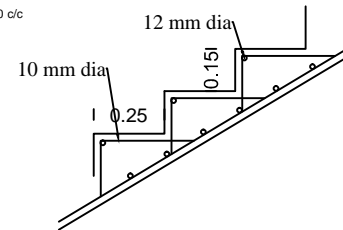
TYPICAL SECTION OF EACH STEP
