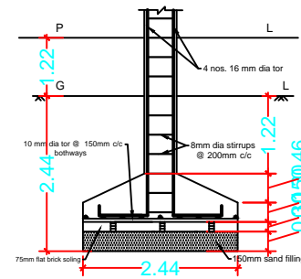
SECTIONAL VIEW OF ISOLATED FOOTING FOR COLUMN FOUNDATION SCALE-1:25
