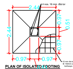
PLAN OF ISOLATED FOOTING FOR COLUMN FOUNDATION SCALE-1:25
