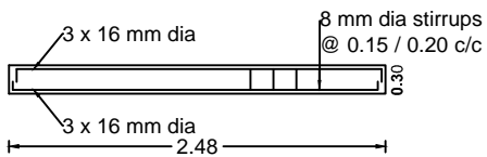
LONGITUDINAL SECTION OF LANDING BEAM
