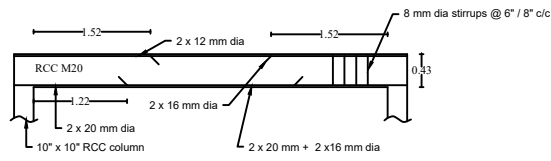
LONGITUDINAL SECTION OF ROOF BEAM
