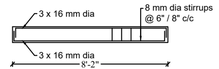
LONGITUDINAL SECTION OF LANDING BEAM
