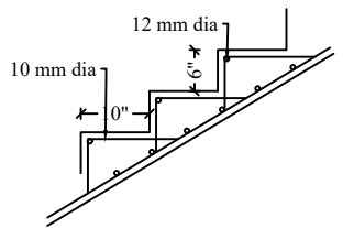
TYPICAL SECTION OF EACH STEP
