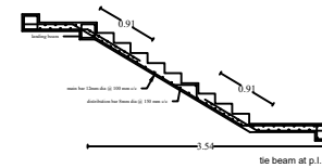
LONGITUDINAL SECTION 1ST FLIGHT
