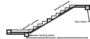
LONGITUDINAL SECTION 2ND FLIGHT
