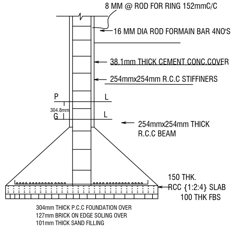
CEOSS SECTION OF R.C.C STIFFINERS
