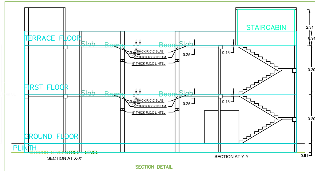
SECTION DETAIL
