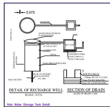
Rain Water Storage Tank Detail
