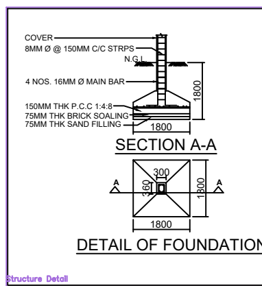
Structure Detail
