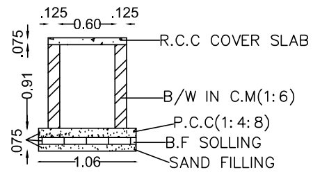
SECTION OF DRAIN SLOPE OF DRAIN=1:200
