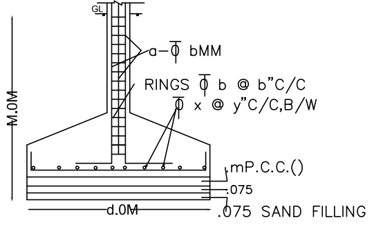
SECTION ON A-A SCALE= 1:50
