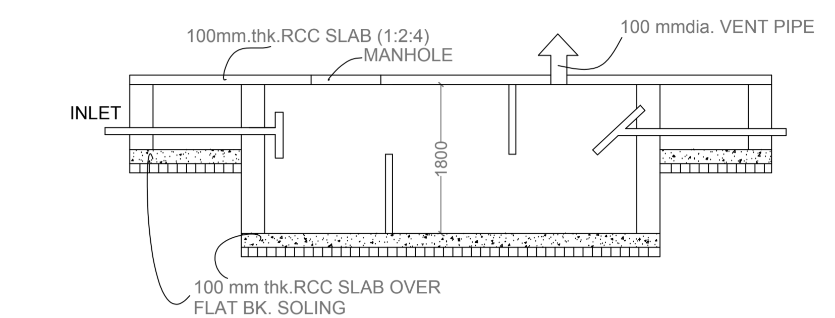
SECTION SCALE 1:50 SEPTIC TANK DETAILS
