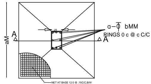
PLAN OF COLUMN FOUNDATION SCALE= 1:50
