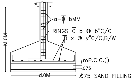
SECTION ON A-A SCALE= 1:50
