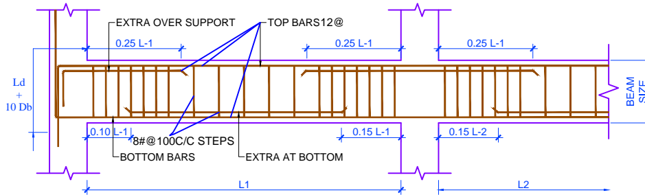
TYPICAL DETAILS OF BEAMS REINFORCEMENT
