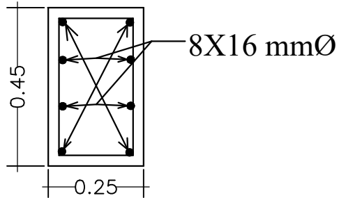
SECTION OF COLUMN. - C1
